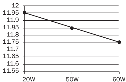
Output Voltage vs. Load at 120V
