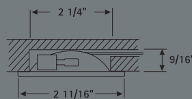
RECESSED MOUNT
