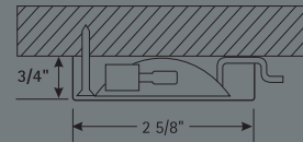
SURFACE MOUNT
