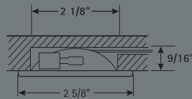
RECESSED MOUNT
